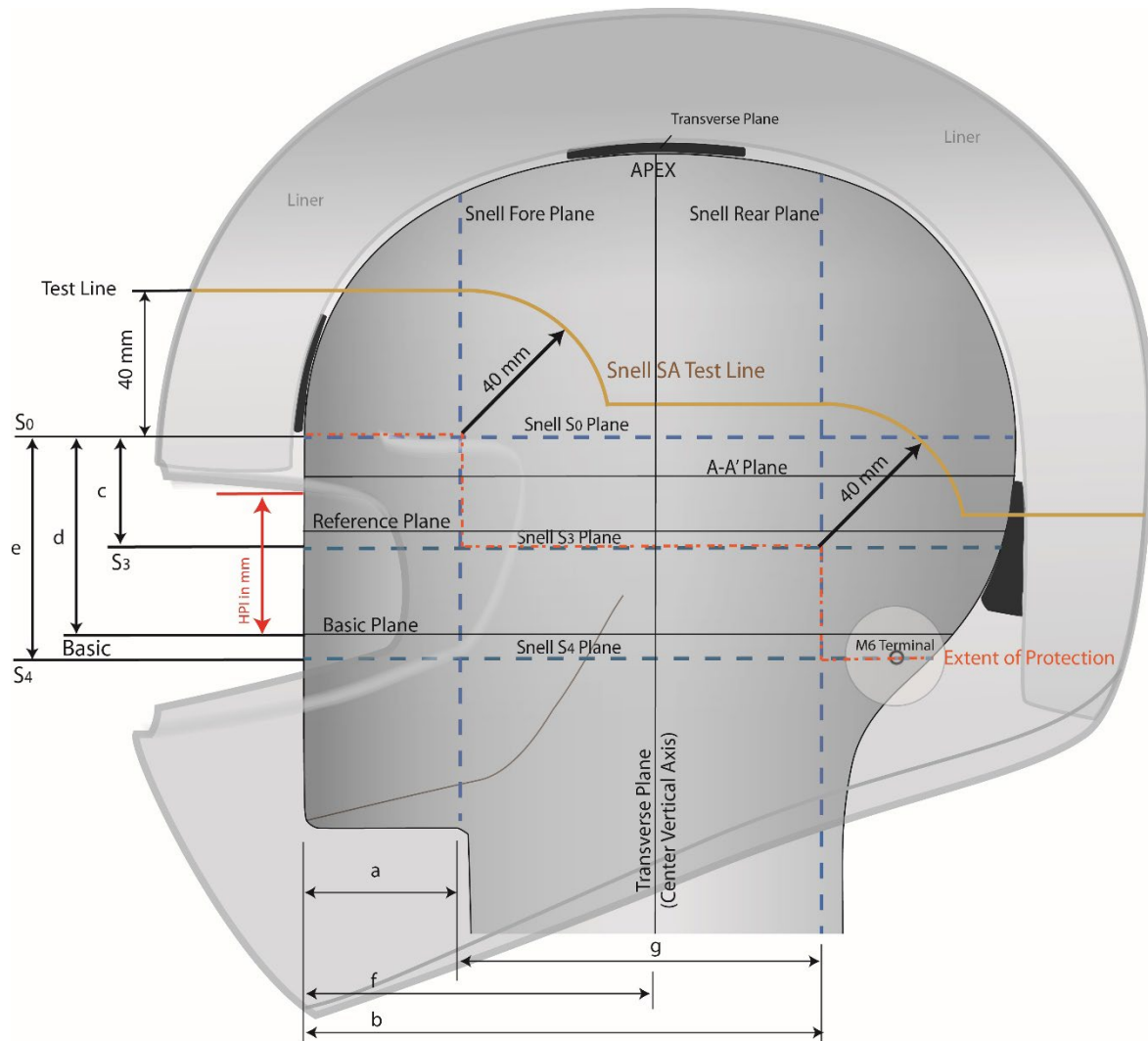
ISO DIS 6220-1983/EN960 Head Form
